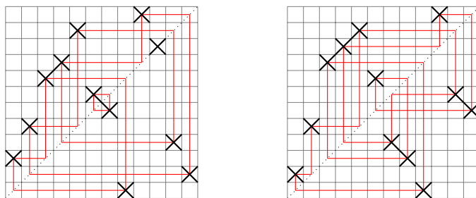
Fig. 2: Two permutations 3 5 8 9 11 7 6 1 12 10 4 2 and 2 5 9 10 11 8 4 3 1 12 7 6 in \mathcal{S}^{+-} and their cycle structure.
