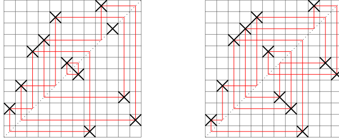
Fig. 2: Two permutations 358911761121042 and 259101184311276 in \mathcal{S}^{+-} and their cycle structure.
