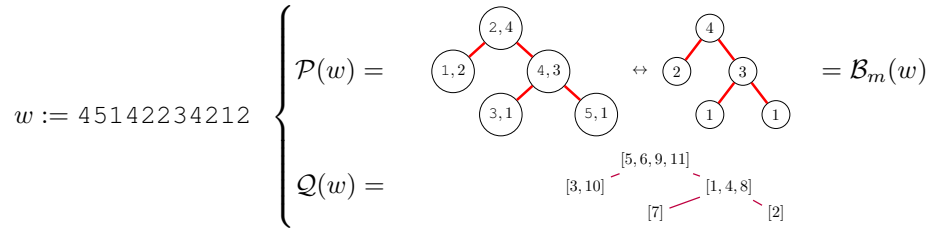
Figure 1: We start by considering the packed word 45142234212, and insert it in a BSTM by the algorithm \mathcal{P} ; that give us \mathcal{P}(45142234212) above in the middle. On the right, there is the BTM ( \mathcal{B}_m(w) ) associated with the BSTM ( \mathcal{P}(w) ) of \mathbf{WQSym}/\equiv_t . At the top of the figure there is the \mathcal{P} -symbol given by \mathcal{P} or \mathcal{B}_m and below the \mathcal{Q} -symbol is given by \mathcal{Q} .
