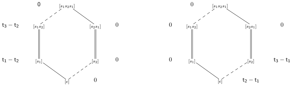
Fig. 2: A class and its image under s_1 .
