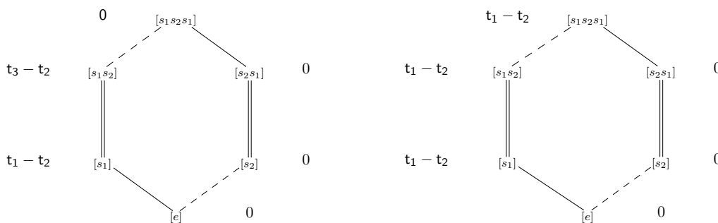
Fig. 3: Non-unique flow-classes
