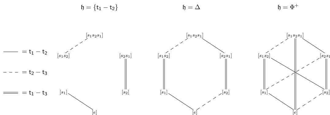
Fig. 1: Hessenberg graphs in type A_2
