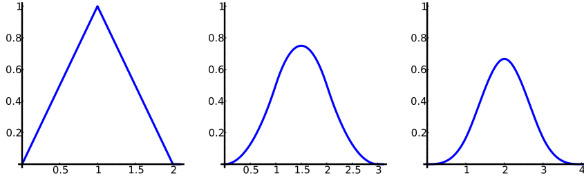
Figure 2: The cardinal B -splines B_2 , B_3 , and B_4 .
