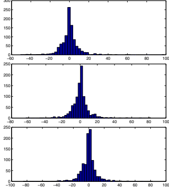
Fig. 4. Histogram for k = 50, 140, 200 of the state estimation error of x_1 , respectively.
