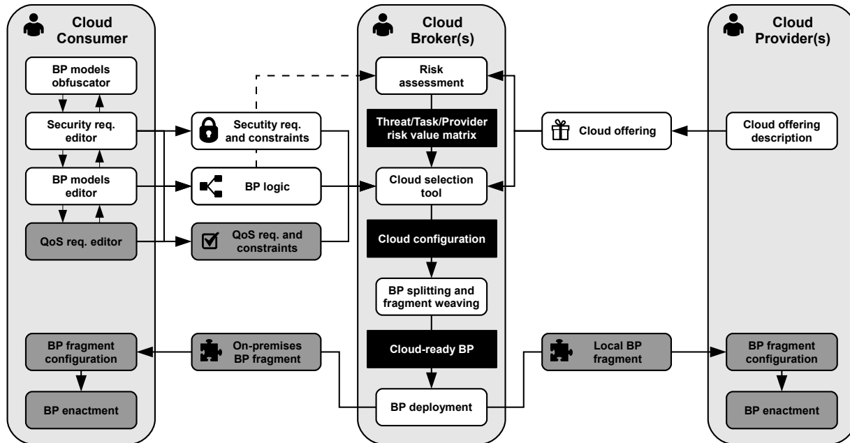
Fig. 2. Architecture
