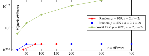
Figure 3: Number of table queries divided by number of points.
