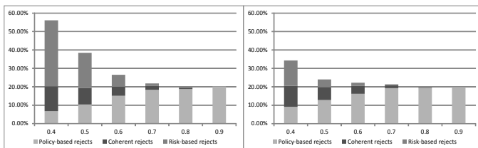
Fig. 5: Ratio of rejected requests in relation to a threshold, for a policy-rejection rate of 20%
