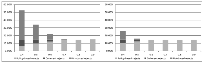
Fig. 4: Ratio of rejected requests in relation to a threshold, for a policy-rejection rate of 15%
