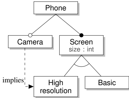
Figure 1. A sample FM for a product line of phones
