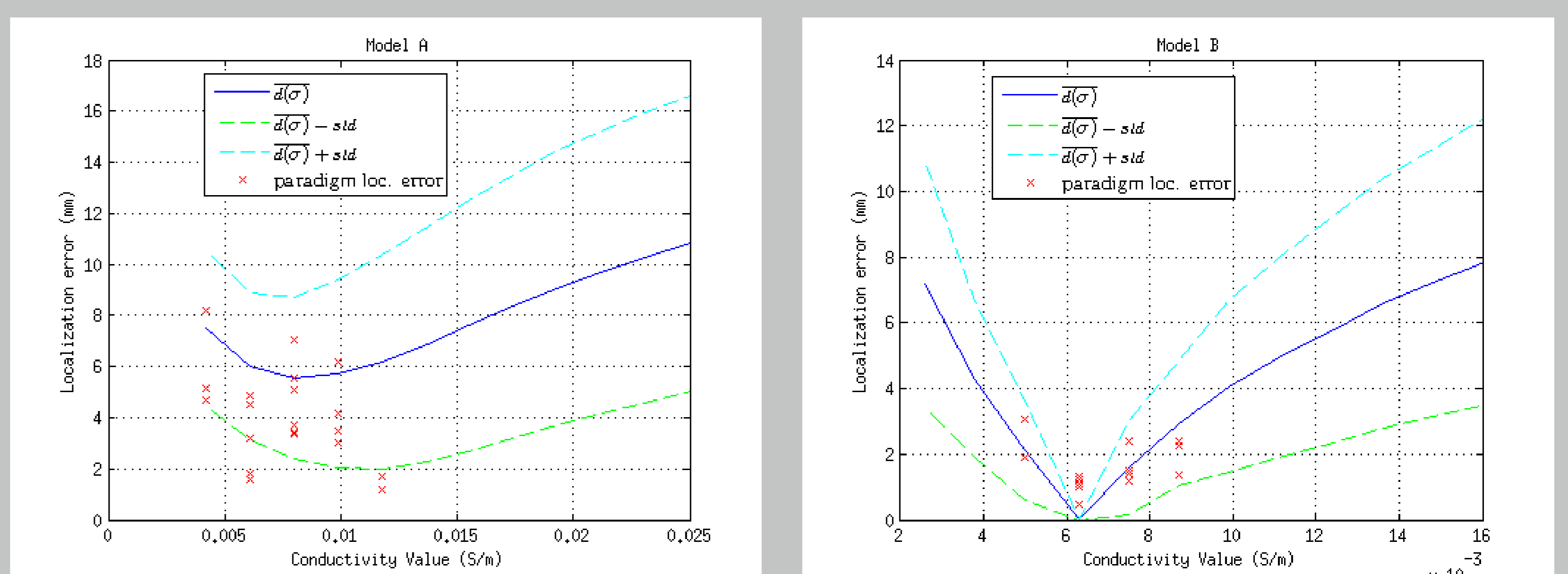
Figure 1 : Plot of localization errors across evenly spread conductivity values for the two test models. The red x symbols indicate the localization error for the 20 manually selected paradigms. The blue line indicates the mean localization errors for 1000 randomly placed sources.
