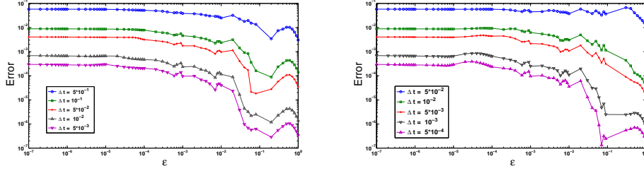
FIG. 4.5. The error between DS computed for \Delta t = 10^{-3} and DS computed for a range of \Delta t , as functions of \varepsilon (log scale). Left: equilibrium initial data (4.1). Right: non equilibrium initial data (4.5).
