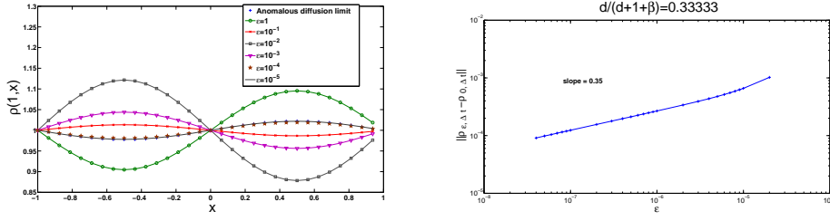
FIG. 4.4. Left: For \Delta t = 10^{-1} , the densities given by DS for a range of \varepsilon and by adiff. Right: For \Delta t = 10^{-1} , the error between DS and the adiff as a function of \varepsilon (log scale).
