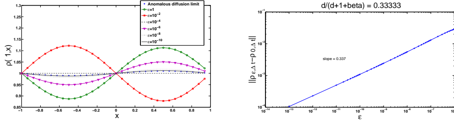
FIG. 4.2. left: For \Delta t = 10^{-3} , the densities given by the MMS scheme for a range of \varepsilon and the anomalous diffusion limit given by the adiff scheme. Right: For \Delta t = 10^{-3} , the error between the MMS scheme and the DSA scheme as a function of \varepsilon (log scale).
