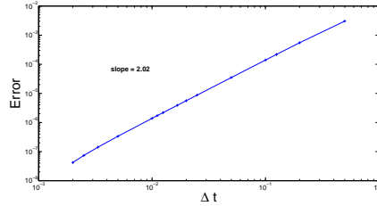
FIG. 4.3. For \epsilon = 1 , the error between DS computed for \Delta t = 10^{-3} and DS computed for a range of \Delta t \in [2 \times 10^{-3}, 0.5] (log scale).
