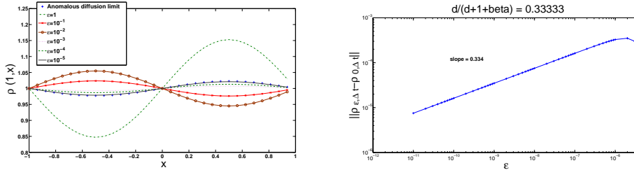
FIG. 4.1. Left: For \Delta t = 10^{-1} , the densities given by IS for a range of \varepsilon and by adiff. Right: For \Delta t = 10^{-1} , the error between the densities given by IS and by adiff as a function of \varepsilon (log scale).
