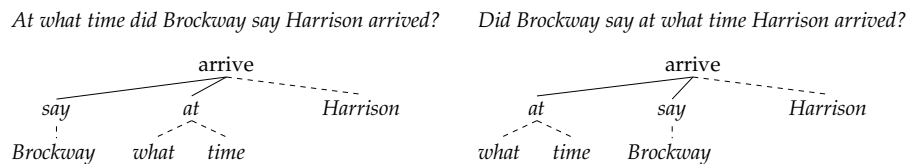
Figure 12 Ordered derivation trees for the sentence (12). Dotted lines indicate substitutions and plain lines adjunctions. Schabes and Shieber’s Outermost Predication principle rules out derivation tree on the left hand side.
