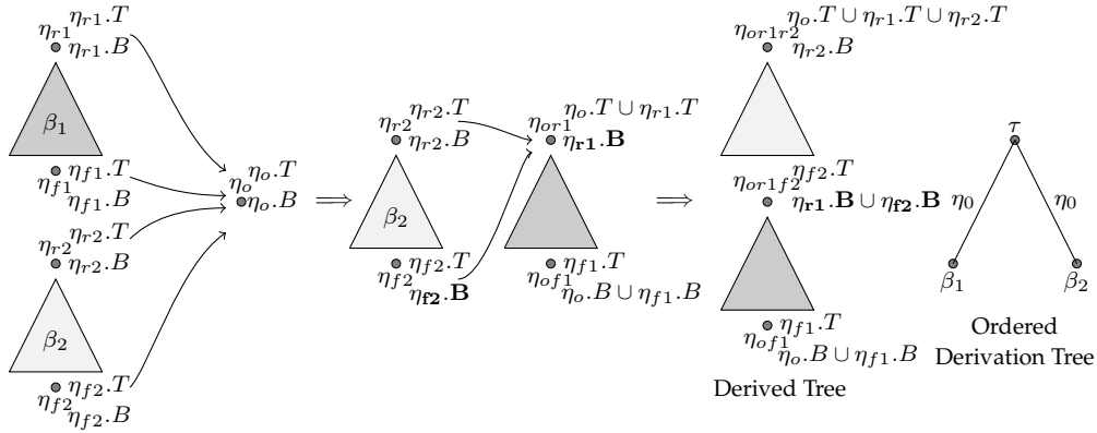
Figure 11 Independent derivation and Feature Unification. The unifications performed by the independent adjunction of \beta_1 and \beta_2 to \eta_o are the same as those that would be performed by a dependent adjunction of \beta_2 to \beta_1 and of the resulting derived tree to \eta_o . Crucially in the independent derivation, although both \beta_1 and \beta_2 adjoin to \eta_o , the adjunction of \beta_2 requires access to the feature structure of the root of \beta_1 ( \eta_{r2}.B \cup \eta_{r1}.B ).
