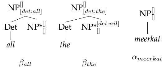
Figure 6 A toy FB-TAG. For the sake of clarity, feature structures are abbreviated.
