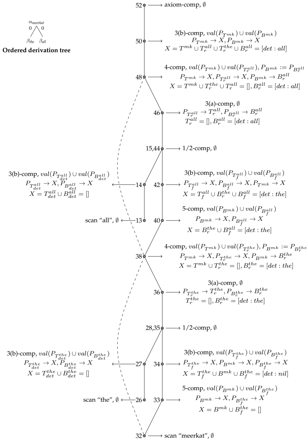
Figure 4 Feature unifications in independent derivation of "all the meerkats" (prediction rules are abbreviated).
