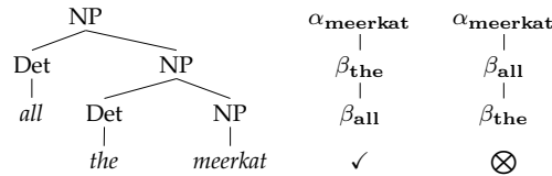
Figure 9 The derived tree (left), the successful standard derivation tree (middle) and the failed dependent derivation tree (right) for “all the meerkats”.
