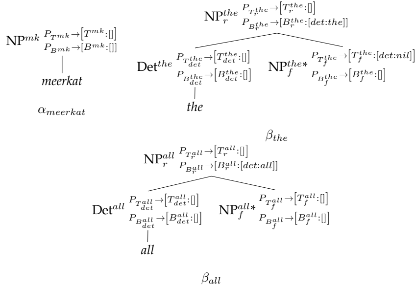
Figure 1 A feature-based Tree-Adjoining grammar.
