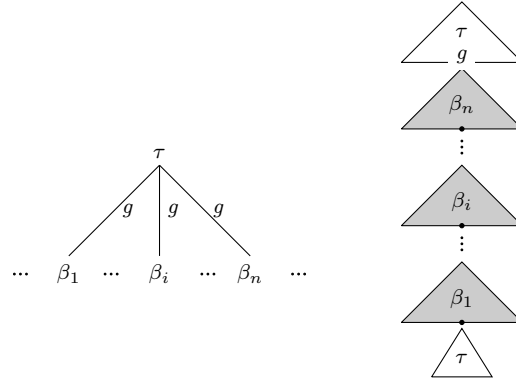
Figure 2 Ordered derivation tree and corresponding derived tree. \tau , \beta_1 , \beta_i and \beta_n are elementary trees. \beta_1 , \beta_i and \beta_n are auxiliary trees which all adjoin at the address g in the elementary tree \tau .
