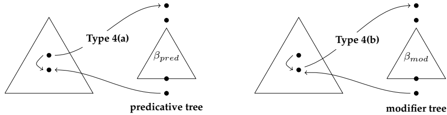
Figure 5 LIG variant of TAG for Schabes and Shieber's Extended derivation. The top and bottom components of the nodes are presented by \bullet . Type 4(a) transitions support dependent, and Type 4(b) independent derivations.
