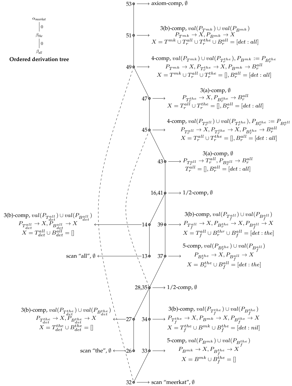
Figure 3 Feature unifications in dependent derivation of "all the meerkats" (prediction rules are abbreviated).
