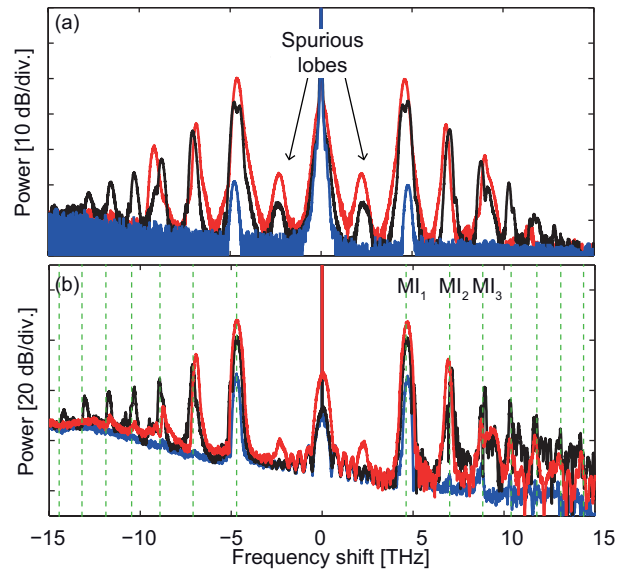
FIG. 7. (Color online) Spectra recorded at the output of fibers A, B and C (we use the same color label than in Fig. 5): (a) Experiments; (b) Numerical simulations which include higher-order dispersions \beta_3 = 5.6 \times 10^{-41} s 3 /m, \beta_4 = -1 \times 10^{-55} s 4 /m and losses \alpha = 5 dB/km.
