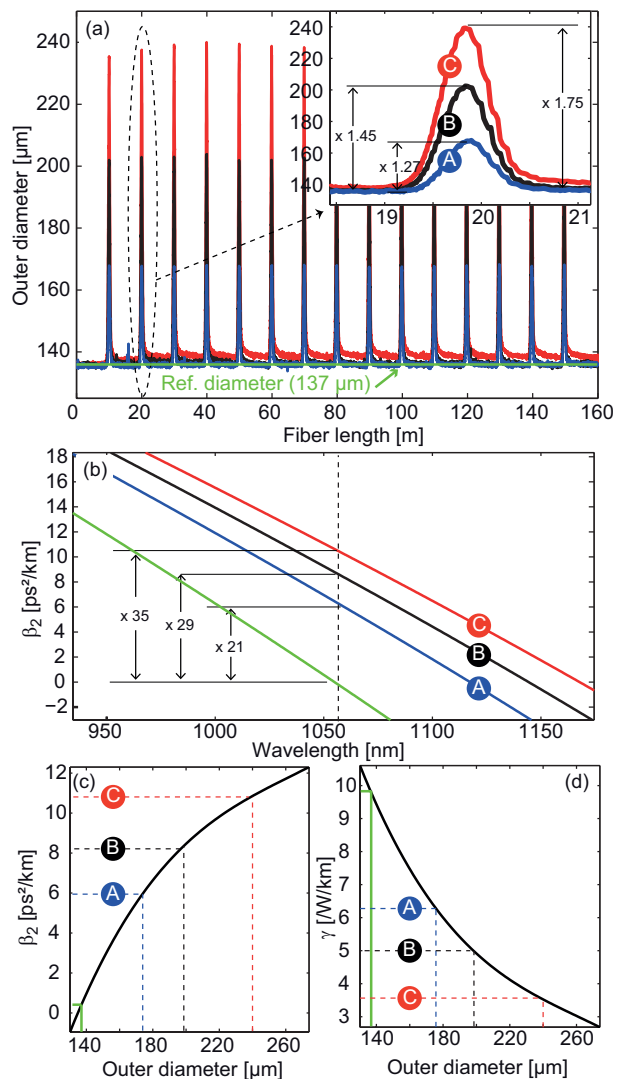
FIG. 5. (Color online) (a) Outer diameter evolution versus fiber length for fibers A, B and C. Inset: Snapshot on one leitmotiv. (b) Calculated GVD curves corresponding to the background diameter (green curve) and the maximum diameter values of fibers A (blue curve), B (black curve) and C (red curve). (c-d) dependence of GVD (c) and nonlinear coefficient (d) on the diameter at wavelength of 1052.5 nm. Curves in (b), (c) and in (d) calculated from Ref. [26] with d/\Lambda = 0.48 and \Lambda_{min} = 3.445 \mu\text{m} .
