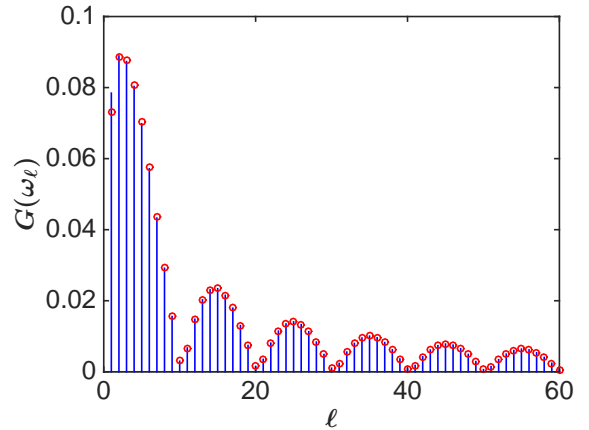
FIG. 3. (Color online) MI gain for \omega = \omega_\ell as a function of \ell ; Red circles, estimated gain given by (20). Parameter values are \beta_{av} = 1 , Z = 1 , \gamma_{av} = 1 , P = 1 , \beta_m = 0.1 .
