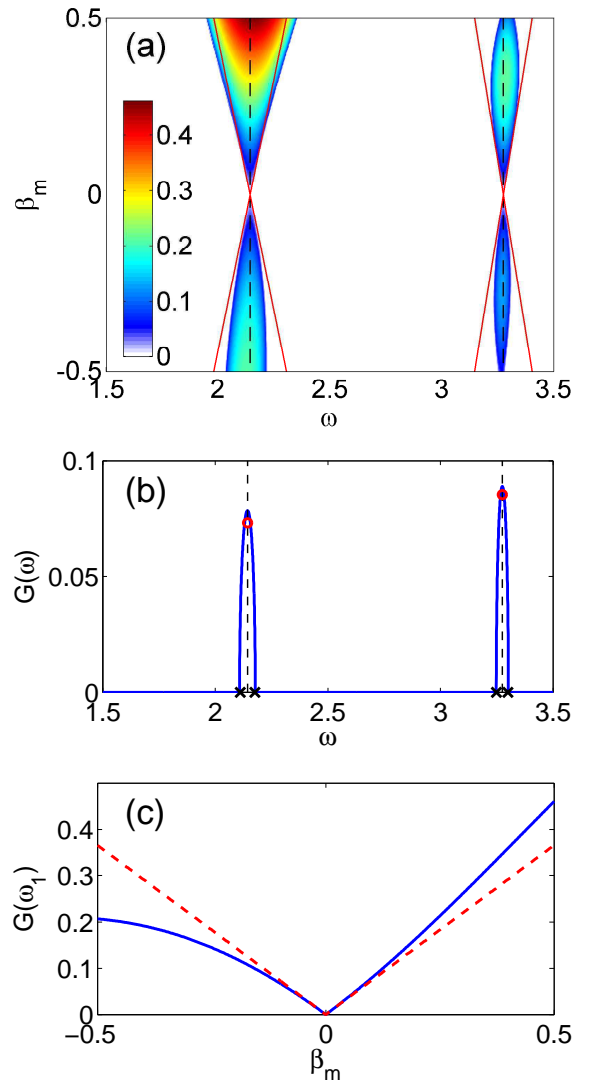
FIG. 2. (Color online) (a) Color level plot of the gain G(\omega, \beta_m) = \ln(\max\{|\lambda_+|, |\lambda_-|\})/Z in the (\omega, \beta_m) plane, for \beta_{av} = 1 , Z = 1 , \gamma_{av} = 1 and P = 1 . The dashed black lines corresponds to the tips of the Arnold tongues (9) at \omega = \omega_1 = 2.1433 and \omega_2 = 3.2748 . The solid red lines corresponds to the gain bandwidth, which can be computed from Eq. (19). (b) MI gain for \beta_m = 0.1 ; Red circles, estimates of maximum gain from Eq. (18); Black crosses, estimates of the bandwidth (19). (c) Solid blue curve, MI gain for \omega = \omega_1 ; Dashed red curve, approximation of maximum gain from Eq. (18).
