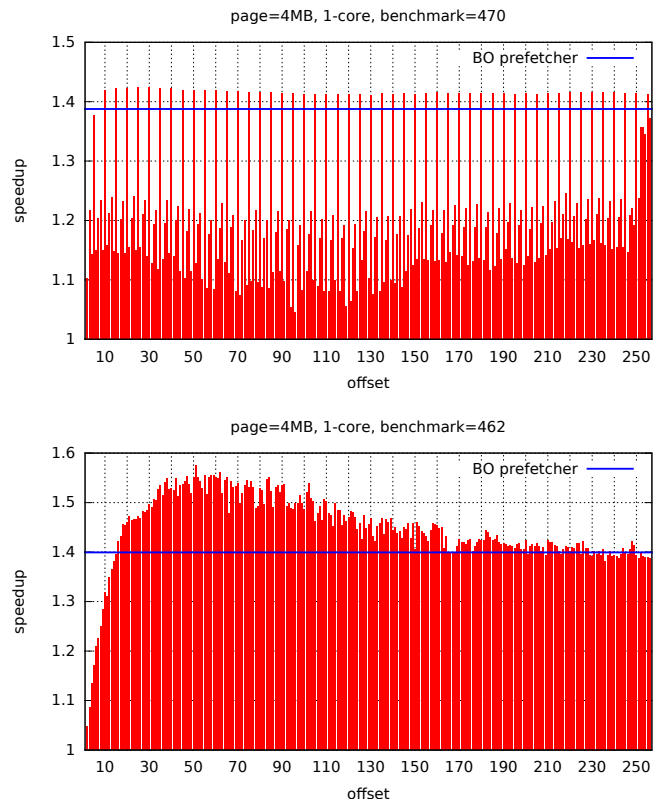
Figure 8: Fixed-offset prefetching with offset ranging from 2 to 256 on benchmarks 433, 459, 470, and 462 (4MB page, 1 active core).
