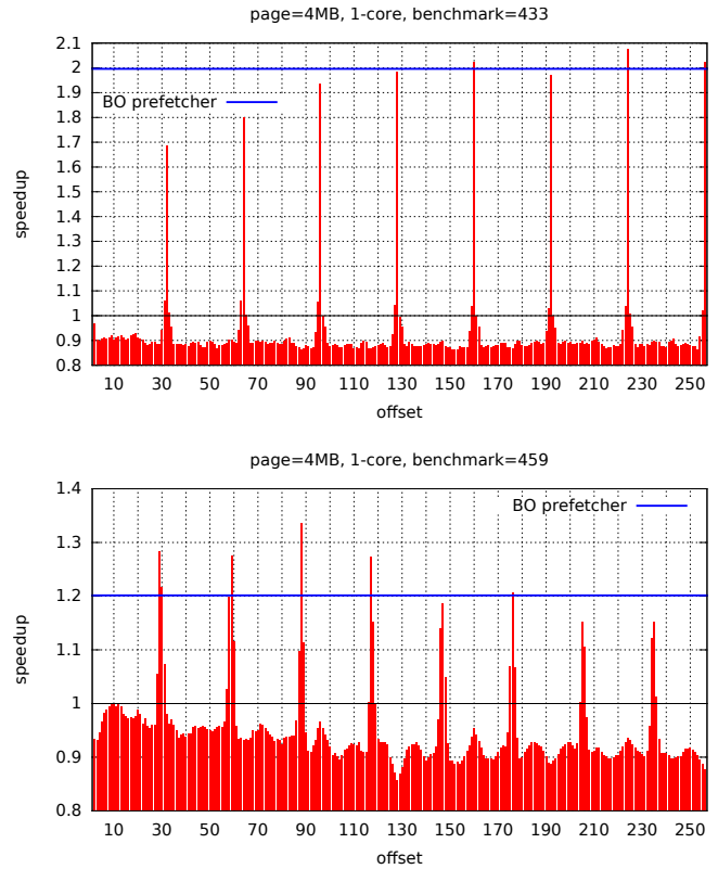
Figure 6: BO prefetcher speedup (relative to next-line prefetching baselines).
