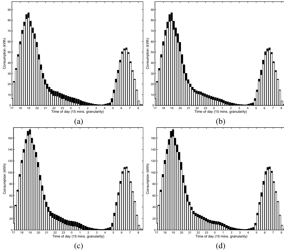
Figure 2: Average of 30-day energy consumption for 40 (top) and 80 (bottom) household units, each using between 10-20 appliances. The consumption of energy from the transformer alone is shown by the white-filled bars whereas the black-filled bars represent the consumption taken from electric vehicles' batteries. Maximising energy consumption from electric vehicles only and maximising energy consumption from electric vehicles considering reducing highest load peaks are shown in the left-hand side and right-hand side of the figure, respectively.
