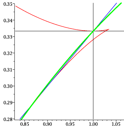
Figure 6: Discriminant loci
