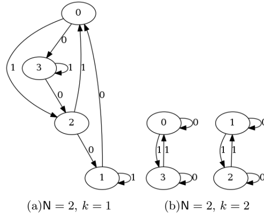
Fig. 2. \mathcal{G}_g of some Caesar ciphers \mathcal{E}_k(x) : \llbracket 0, 2^N - 1 \rrbracket \longrightarrow \llbracket 0, 2^N - 1 \rrbracket, x \longmapsto x + k \pmod{2^N}
