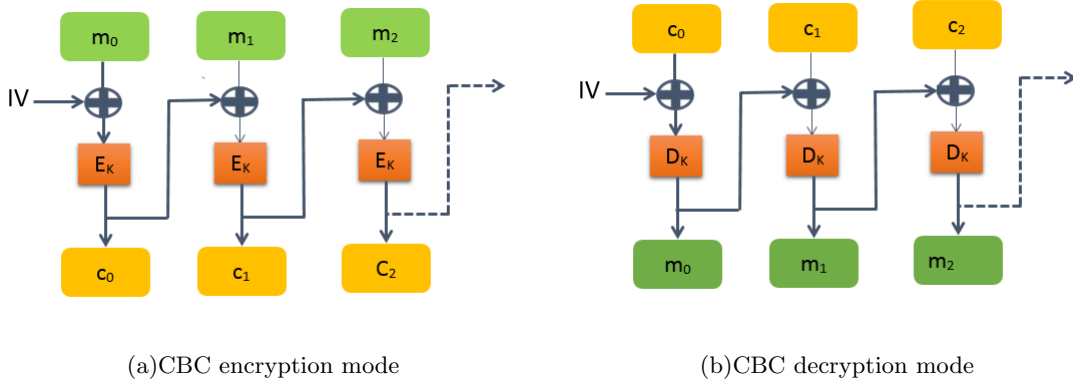
Fig. 1. CBC mode of operation
