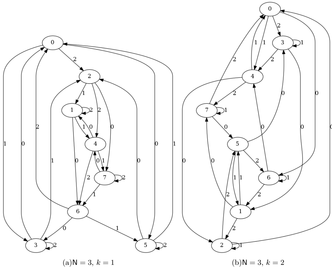
Fig. 3. \mathcal{G}_g of some Caesar ciphers \mathcal{E}_k(x) : \llbracket 0, 2^N - 1 \rrbracket \longrightarrow \llbracket 0, 2^N - 1 \rrbracket, x \longmapsto x + k \pmod{2^N}
