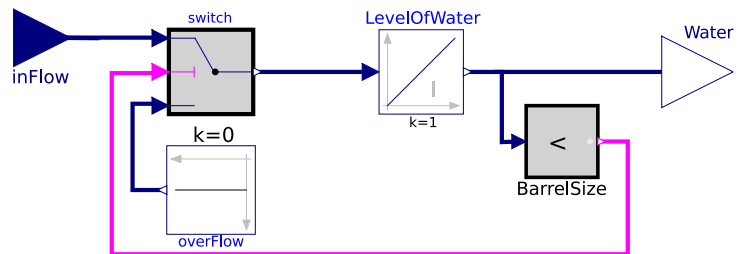
Figure 3: The barrel model viewed in Dymola
