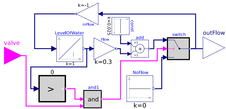
Figure 2: The tank model viewed in Dymola
