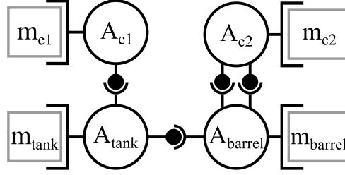
Figure 6: MECSYCO architecture for the barrel-filler factory.
