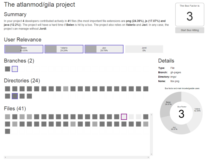
Fig. 5: Bus factor analysis of a file in GiLA
