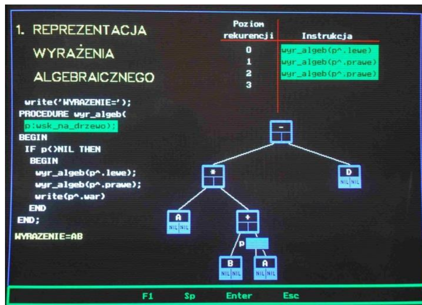
Figure 3: A screen with Package EI – demonstration of a tree data structure
