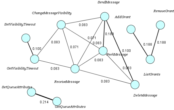
Fig. 5. G_{MessageQueue}^{conv} for MessageQueue.
