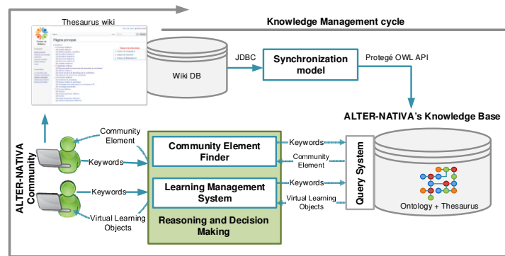
Fig. 2. ALTER-NATIVA's Knowledge Management architecture.
