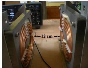
Fig. 4. Transmitter with FLUXTROL 50 ferrite.
