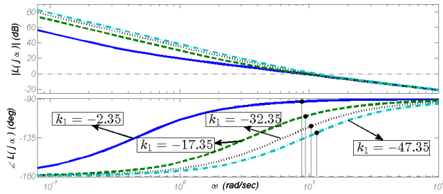
Fig. 9. Bode plot for the loop transfer function L with different values of k_1
