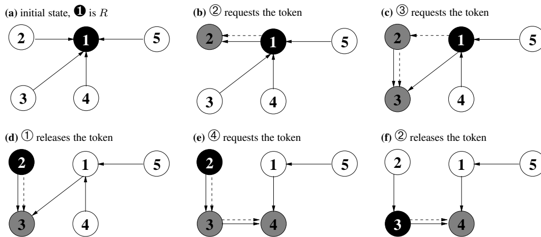
Figure .1: Example of the execution of Naimi and Tréhel's Algorithm
