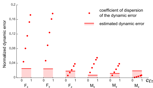
Figure 2: Coefficients of dispersion of the dynamic error and estimated [3].
