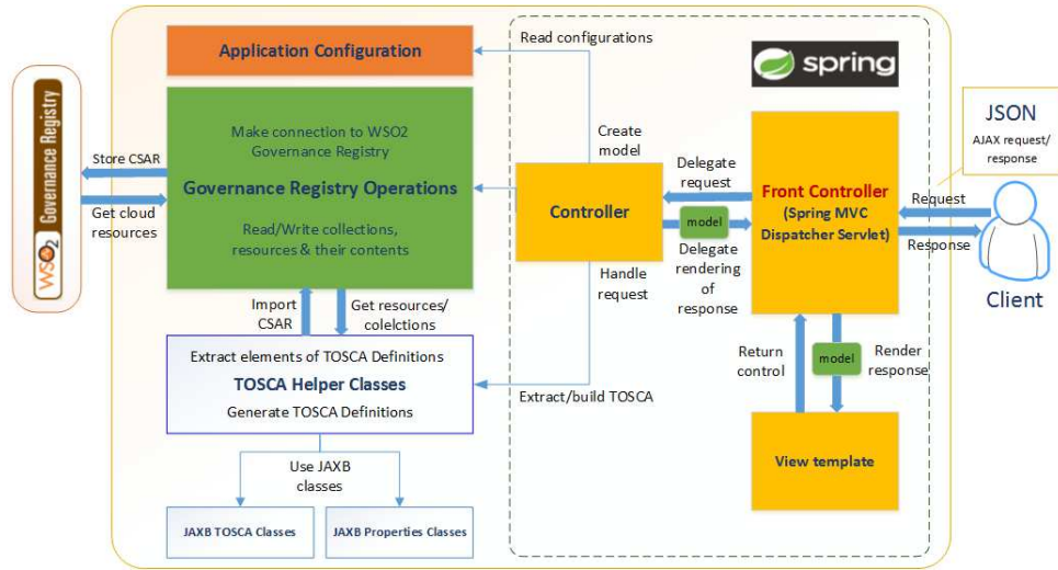
Fig. 2. Cloud REA Model (CREAM) architecture.
