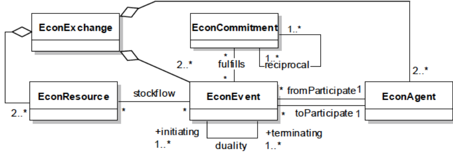
Fig. 1. Excerpt of the REA meta-model and core concepts.
