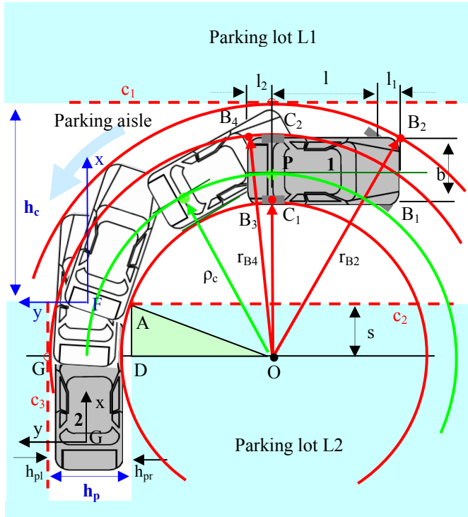
Fig. 2. Geometry of the collision-free perpendicular parking maneuver
