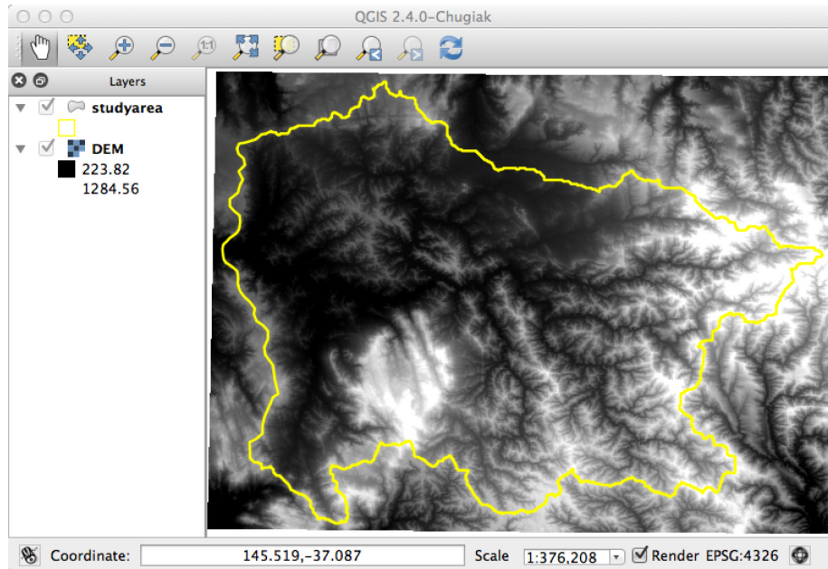
Fig. 3. QGIS visualization of Geoscience Australia DEM acquired for bounding box of study area defined by watershed shapefile.
