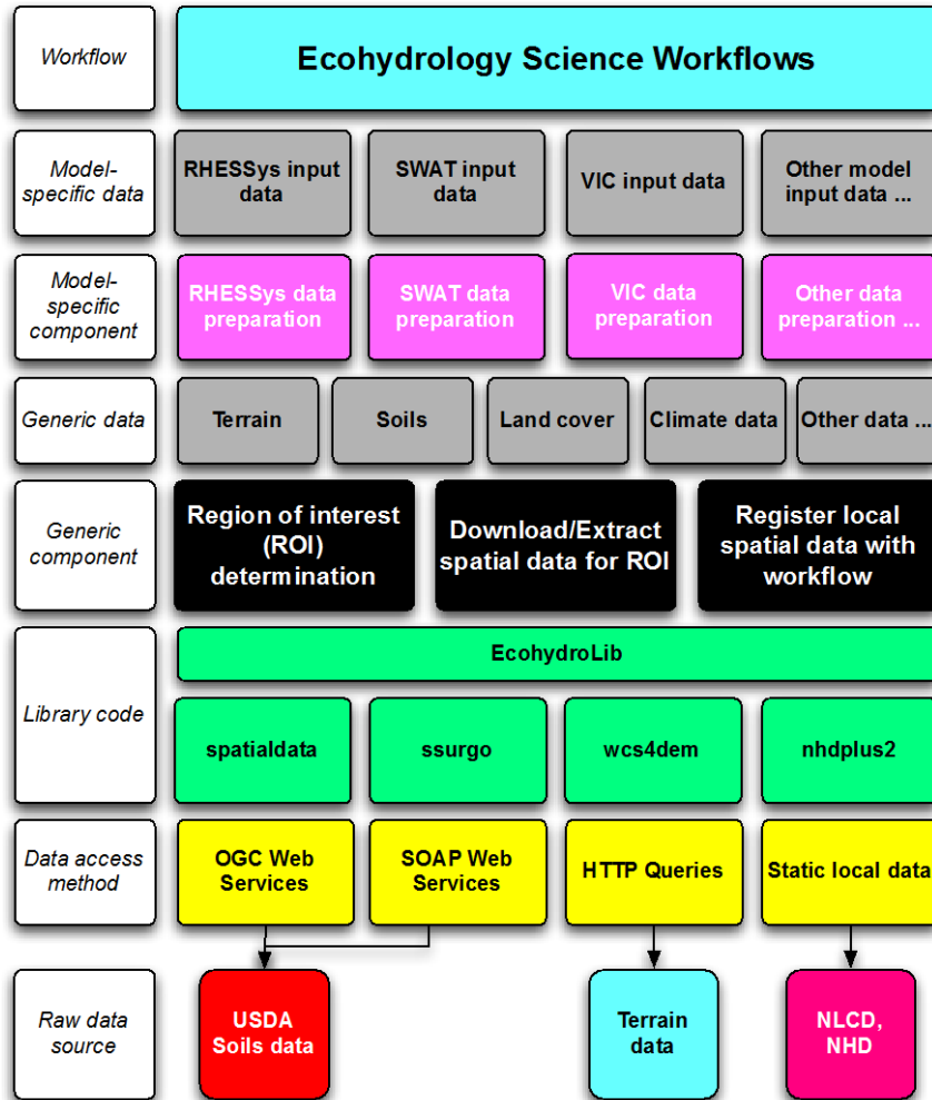
Fig. 1. Illustration of layered architecture of EcohydroLib. Read from the bottom, raw data sources are accessed using web services (yellow), or as static data stored on local files systems (yellow), using library code (green) in EcohydroLib. Generic data acquisition tools (black) are built on top of EcohydroLib library code. These tools yield data in generic formats not specific to any model (grey). Model-specific tools (magenta) use these generic data to produce model-specific input data parameterizations (grey, above magenta). The model specific data make possible ecohydrology modeling science workflows (cyan) whose goal is to answer particular science and management questions.
