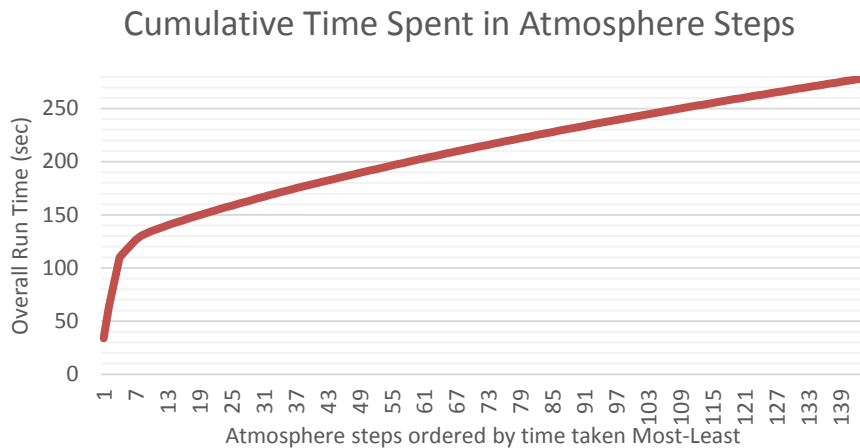
Fig. 8. Cumulative time spent in UM atmosphere steps, ordered by longest time step to shortest. This was performed with a 32 \times 62 decomposition using 4 IO servers each with 16 MPI tasks, for a total of 4096 cores.
