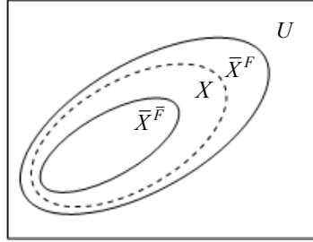
Figure 2. U is finite element universe, X is the finite general element set on U , which has the attribute set \alpha , and X can be shown in broken line. \bar{X}^F is inter inverse P-sets, it has the attribute set \alpha^F , and \bar{X}^F can be shown in real line. \bar{X}^{\bar{F}} is outer inverse P-sets, it has the attribute set \alpha^{\bar{F}} , and \bar{X}^{\bar{F}} can be shown in real line. Inverse P-sets (\bar{X}^F, \bar{X}^{\bar{F}}) is composed of \bar{X}^F and \bar{X}^{\bar{F}} .
