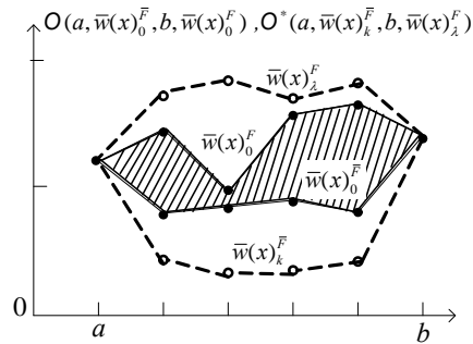
Figure 1. O(a, \bar{w}(x)_0^F, b, \bar{w}(x)_0^F) is information law with two boundary, O(a, \bar{w}(x)_0^F, b, \bar{w}(x)_0^F) is shown in real line; O^*(a, \bar{w}(x)_k^{\bar{F}}, b, \bar{w}(x)_\lambda^F) is the hiding information image of O(a, \bar{w}(x)_0^F, b, \bar{w}(x)_0^F) , and O^*(a, \bar{w}(x)_k^{\bar{F}}, b, \bar{w}(x)_\lambda^F) is shown in
