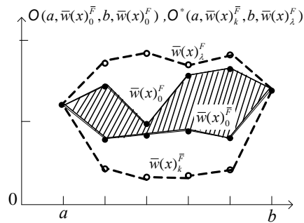
Figure 1. O(a, \bar{w}(x)_0^F, b, \bar{w}(x)_0^F) is information law with two boundary, O(a, \bar{w}(x)_0^F, b, \bar{w}(x)_0^F) is shown in real line; O^*(a, \bar{w}(x)_k^F, b, \bar{w}(x)_\lambda^F) is the hiding information image of O(a, \bar{w}(x)_0^F, b, \bar{w}(x)_0^F) , and O^*(a, \bar{w}(x)_k^F, b, \bar{w}(x)_\lambda^F) is shown in
