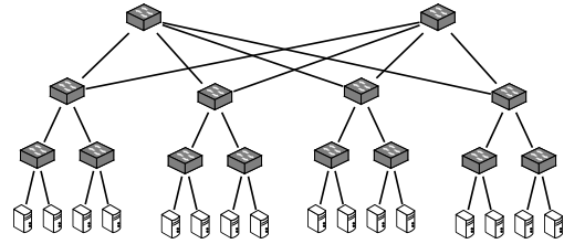
Figure 3. Reference topology.
