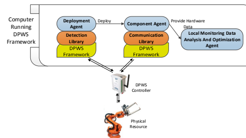
Fig. 4. PRIME Agent environment using a Semi-intelligent Resource
