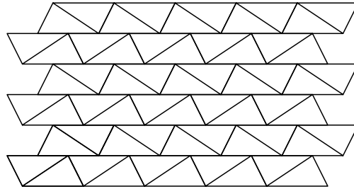
Fig. 59: Tiling with one type of arbitrary triangle but odd rows are reflected.
