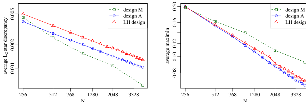
Figure 1. Log-log graph of averaged L_2 star discrepancy (left) and maximin (right) for designs M and A over 100 repetitions.
