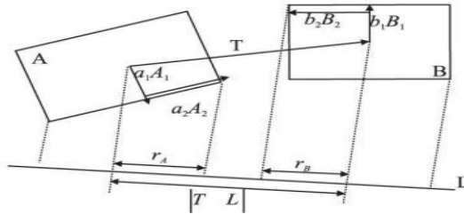
Fig.2.OBB-OBB overlap test
