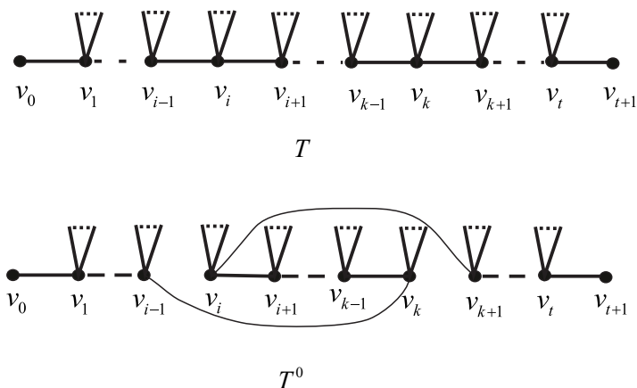
Fig. 1: A new path in T^0 obtained from T by S(v_i, v_k) on the path v_0v_1v_2 \dots v_tv_{t+1} .
