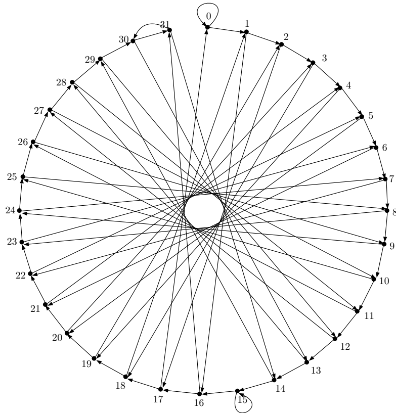
Fig. 9: A spanning 2-diregular biculerian subdigraph \vec{H}_1 of \vec{G}'_6 .
