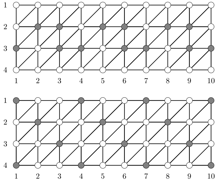
Figure 5: Two identifying codes of T_4 with minimum density 1/3 .
