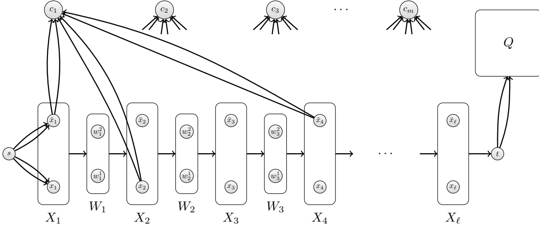
Figure 1: The digraph D , where C_1 = (\bar{v}_1 \vee v_2 \vee \bar{v}_4)
