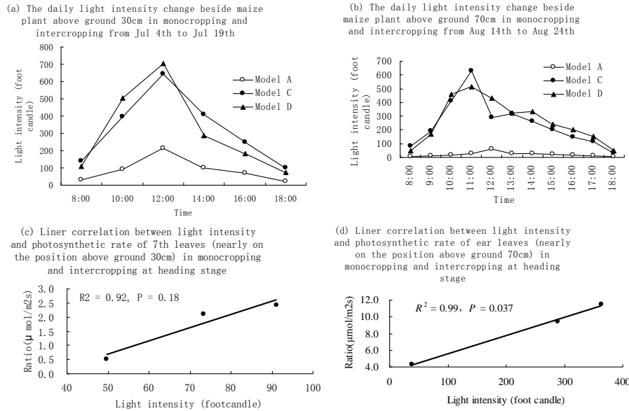
Fig.2. Daily light intensity change beside maize plants above ground 30cm and 70cm and the relationship between light intensity and photosynthetic rate in monocropping and intercropping at heading stage
