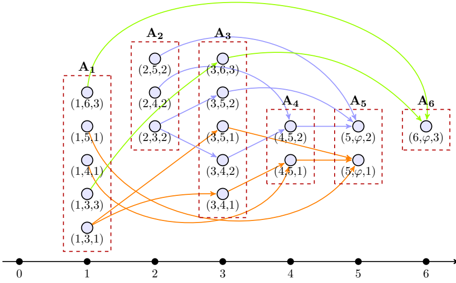
Fig. 12: Simplex Array List for complex in Figure 1 embedded on the number line.
