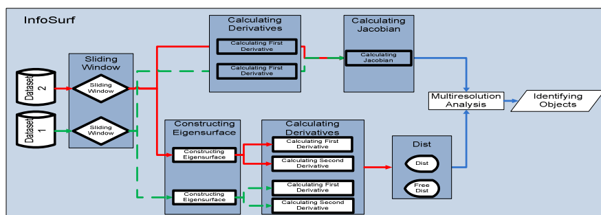
Fig.1. The InfoSurf workflow diagram. This figure shows the flow of data in the algorithm.
