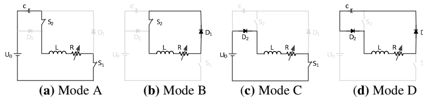
Fig. 6. Operating modes for the topology with capacitor
