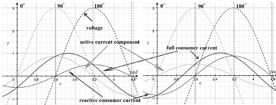
Fig.5. Voltage, active, reactive and full current graphs, where a) \cos\varphi=0,5 ; \varphi=60^\circ ; b) \cos\varphi=0,866 ; \varphi=30^\circ .
