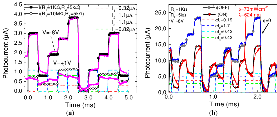
Fig. 7. Multiplexed simulated (symbols), current sources (dash lines) and experimental (solid lines): a) under negative ( R_1=1\text{k}\Omega ; -8\text{V} ) and positive ( R_1=10\text{M}\Omega ; +1\text{V} ) dc bias without any background; b) under negative ( R_1=1\text{k}\Omega ; -8\text{V} ) and red (b) background ( \phi=73\text{mWcm}^{-2} )
