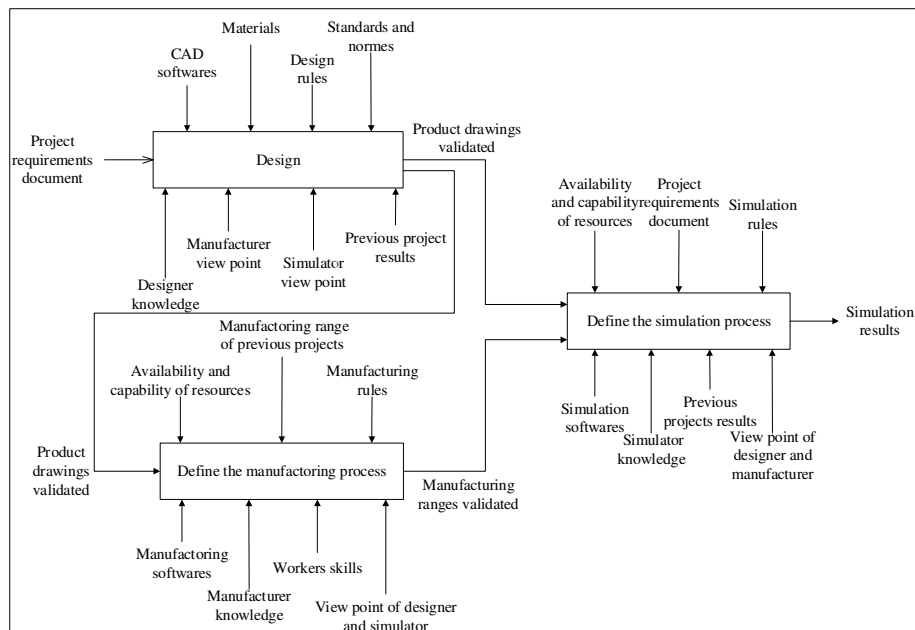
Fig. 4. Digital manufacturing process of tank in digital factory
