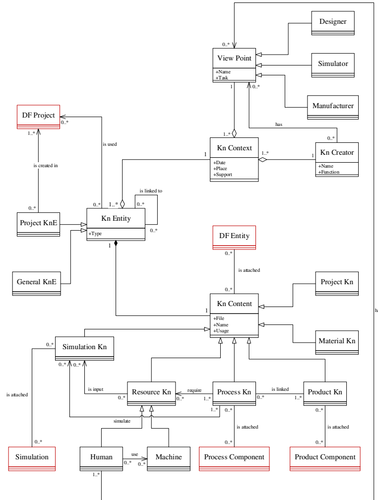
Fig. 3. Conceptual Model
