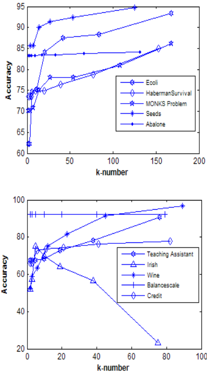
Fig. 3. The line chart of clustering accuracy rate.
