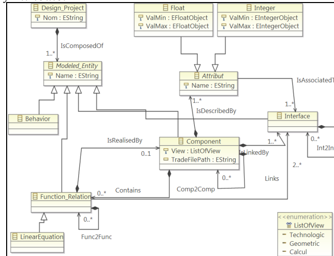
Fig. 3.Current mediator meta-model
